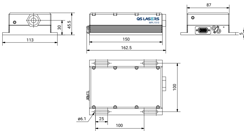
MPL1510 laser head dimensions (in mm)
